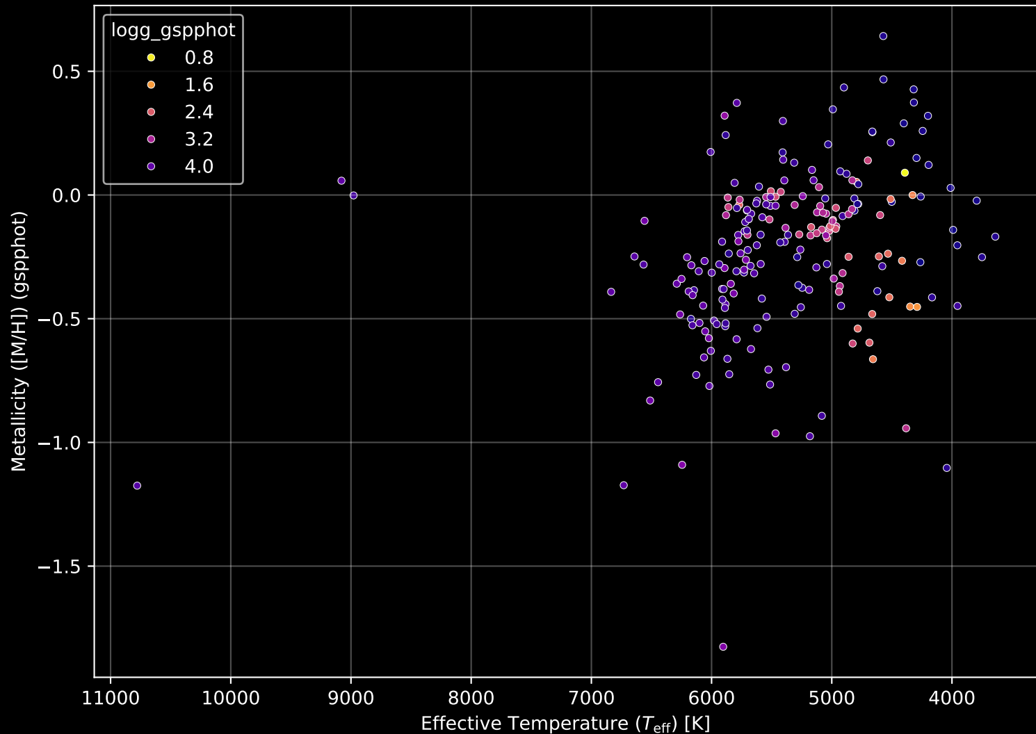
APOGEE DR17 Field: [062-43_MGA] Stellar Population Parameters (n= 214)
