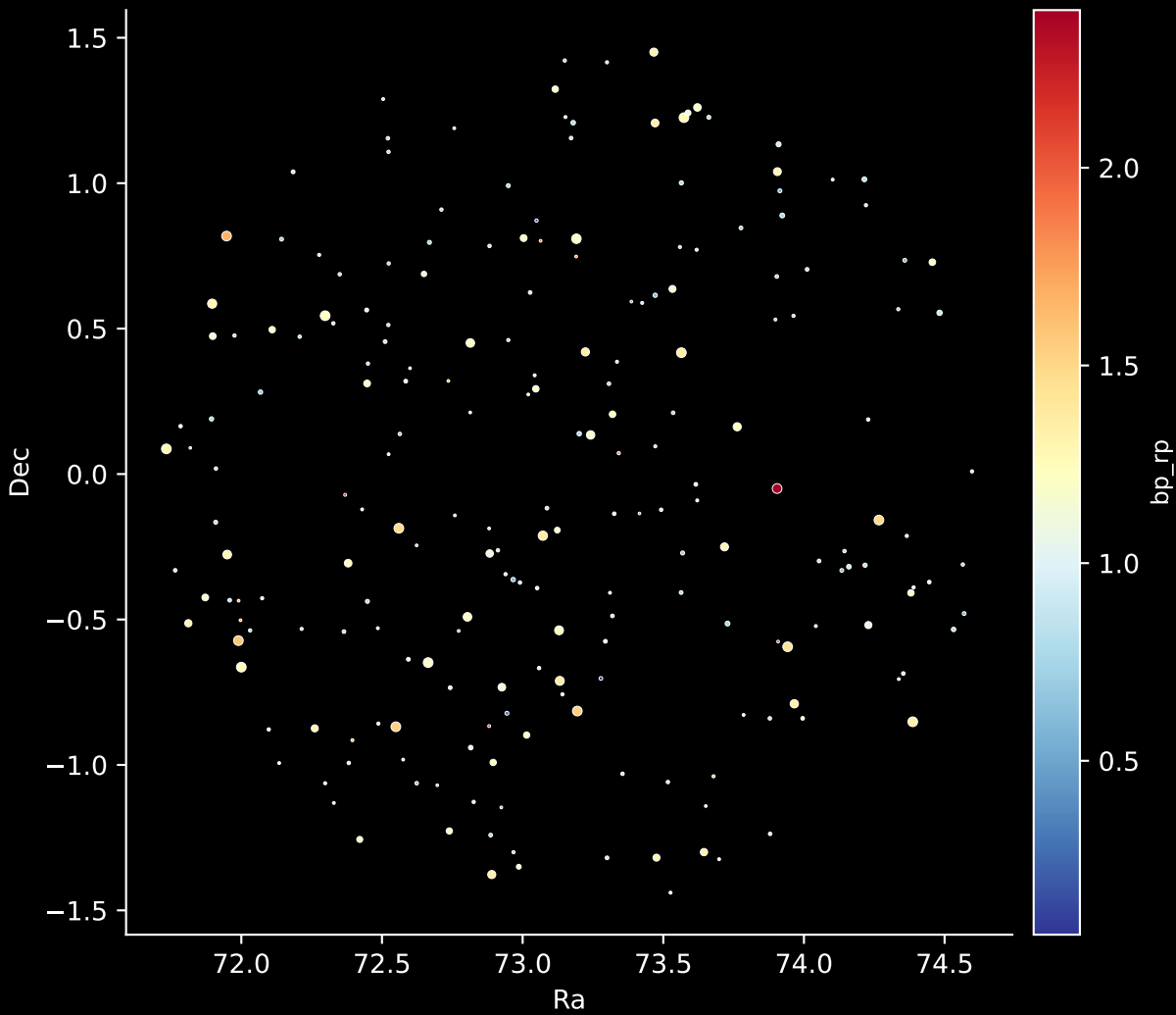
APOGEE DR17 Field: [062-43_MGA] Stars: 214
