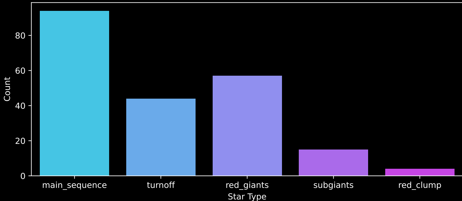
APOGEE DR17 Field: [062-43_MGA] Count plot of Star Type
