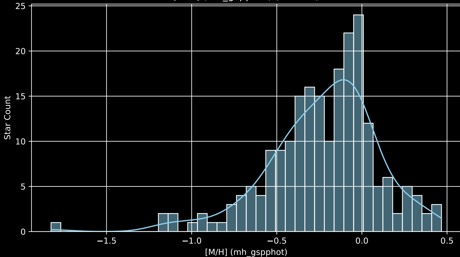
APOGEE DR17 Field: [062-43_MGA [M/H] (mh_gspphot) (n= 213)
