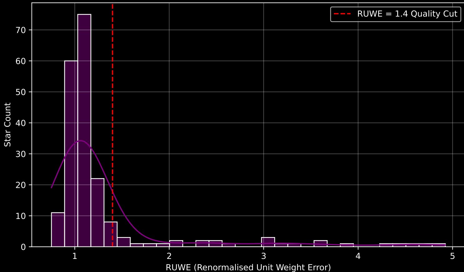
GAPOGEE DR17 Field [062-43_MGA] RUWE Distribution (n= 202)
