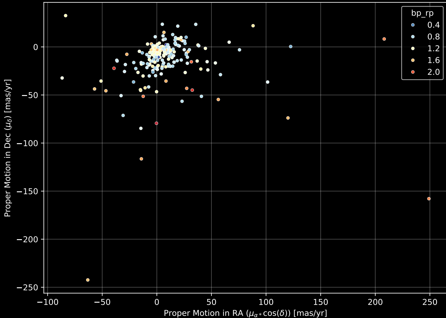
APOGEE DR17 Field: [062-43_MGA] Proper Motion Diagram (n= 214)
