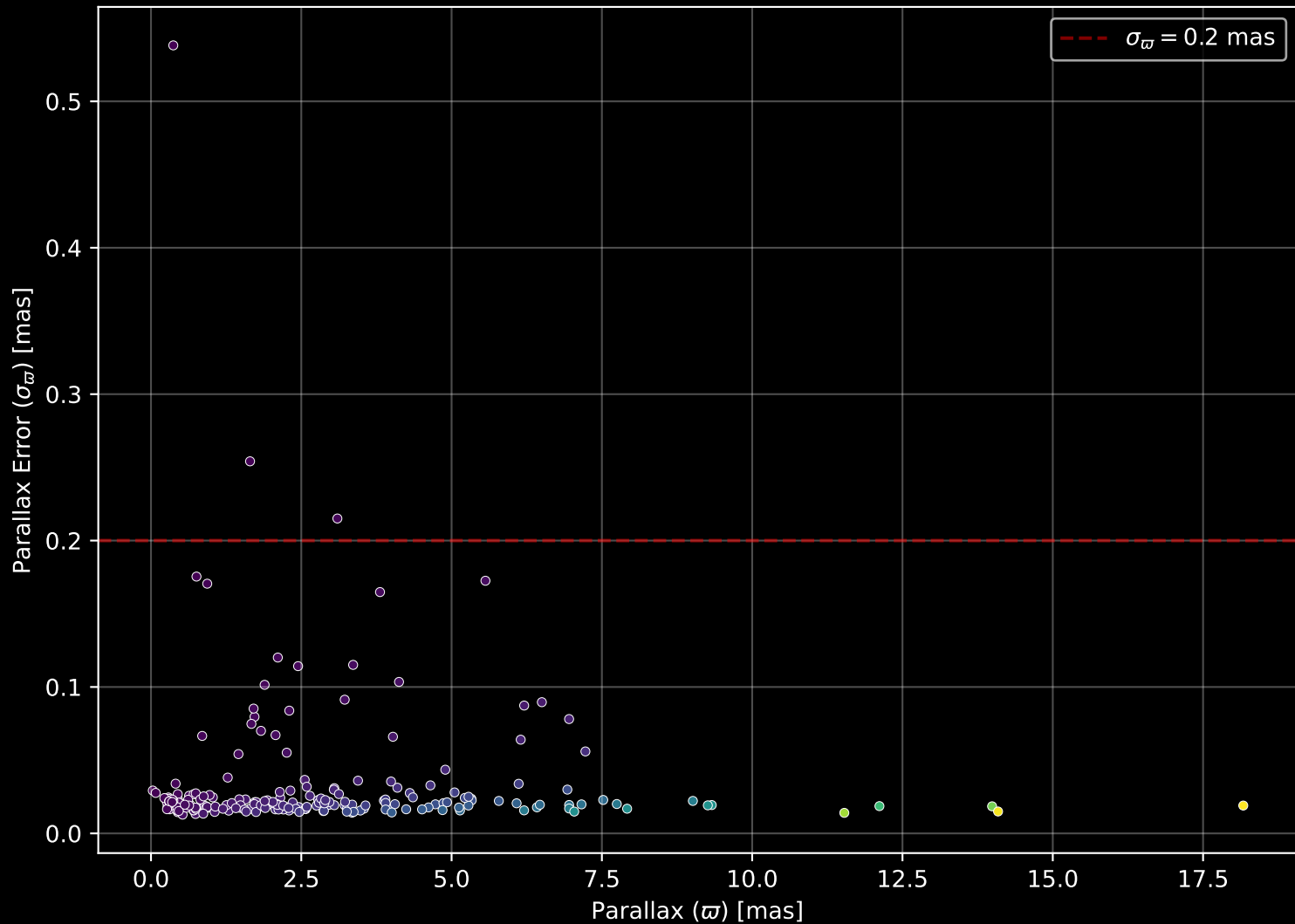
APOGEE DR17 Field: [062-43_MGA] Parallax Quality (n= 214)
